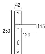
Cod. 01 CC 01 RQ Maniglia con placca \varnothing 8 x 90 Door handle with plate \varnothing 8 x 90
