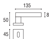
Cod. 177 CC 01 RQ Maniglia con placca \varnothing 8 x 90 Door handle with plate \varnothing 8 x 90
