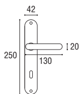
Cod. 143 OL 01 Maniglia con placca \varnothing 8 x 90 Door handle with plate \varnothing 8 x 90
