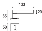
Cod. 186 CC 01 RQ Maniglia con placca \varnothing 8 x 90 Door handle with plate \varnothing 8 x 90
