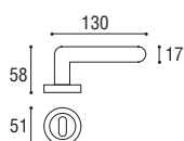
Cod. 10 CC 01 Maniglia con placca \varnothing 8 x 90 Door handle with plate \varnothing 8 x 90
